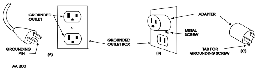
Figure 1. Grounding methods
