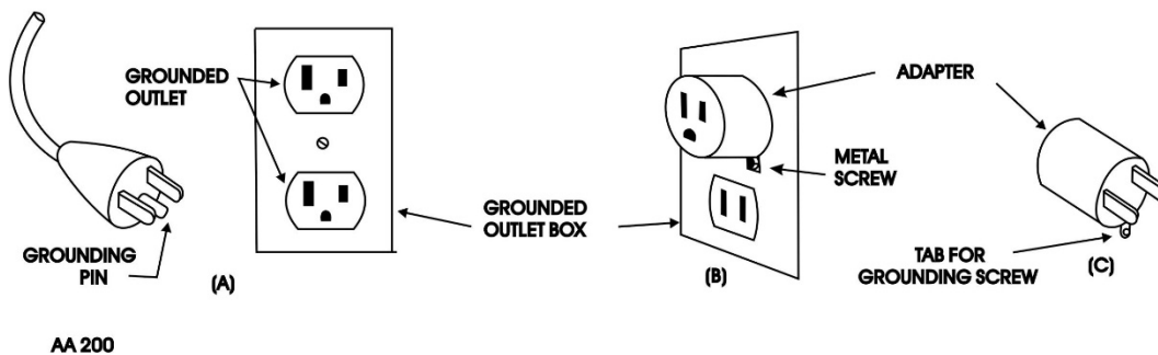
Figure 1. Grounding methods
